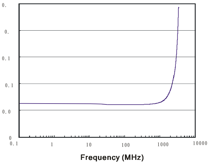
Capacitance (pF):
