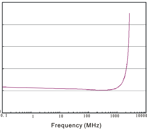
Capacitance (pF):
