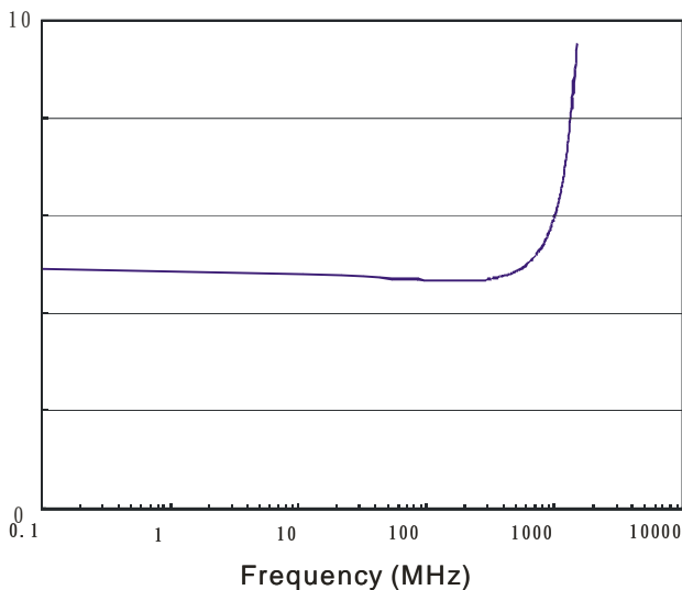
Capacitance (pF):
